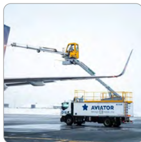
丹麦 Vestergaard Company A/S大象除冰车 Elephant Series De-icers, Vestergaard Company A/S
